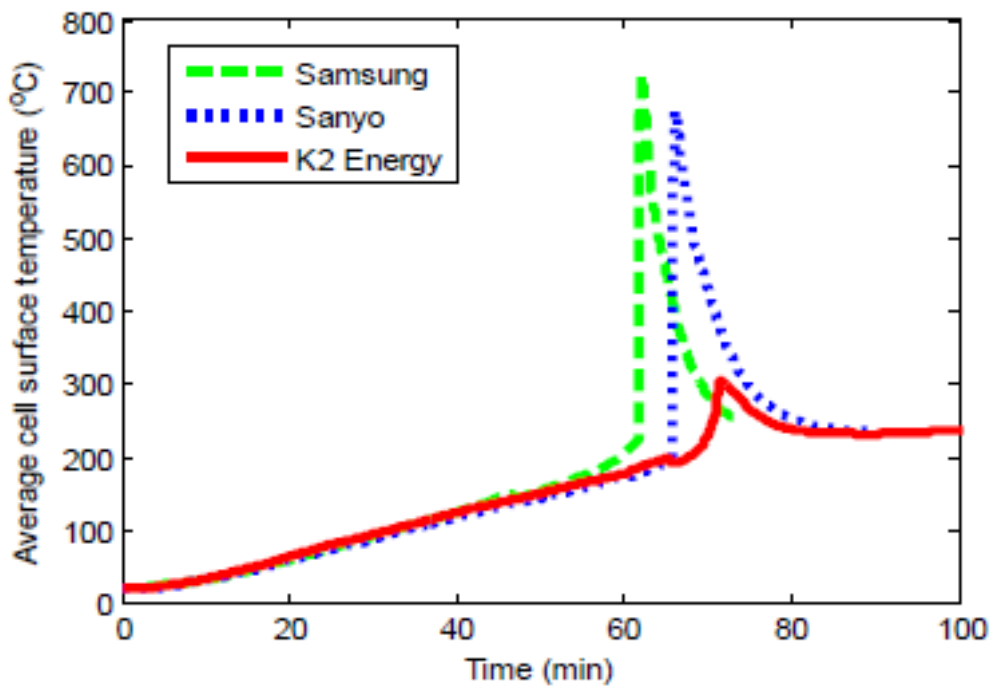
The battery cell surface temperature during external heating (oven) abuse test, showing the temperature rise upon external heating and the rapid temperature peak due to thermal runaway for two types of cobalt based cells (Samsung and Sanyo) and for a lithium iron phosphate cell (K2 Energy). All three cells are of the 18650 type. Reprinted with permission of F. Larsson [3].
